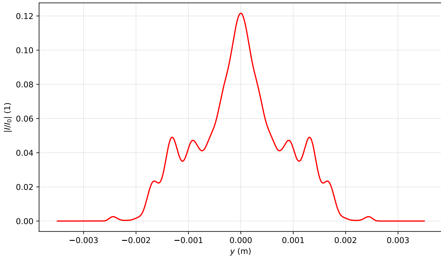
Intensity profile I(x=0, y, z=3.344)/I_0 , P_{in}=5.5P_{cr} , artificial time
